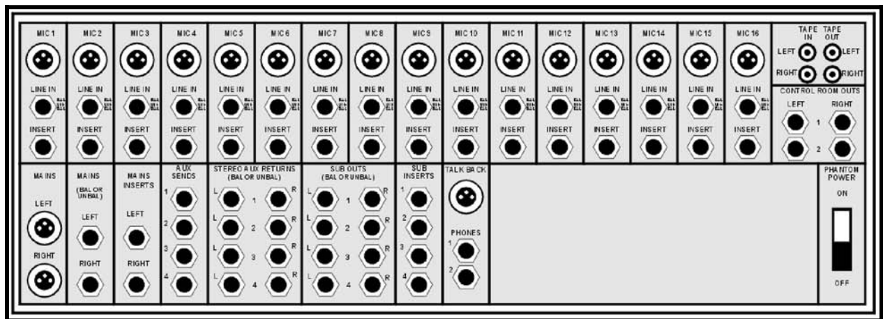
Figure 5 Advanced Mixer Rear Panel View
